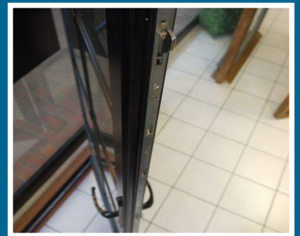
Multi Point Locking Hook Locks Secure Into The Frame
